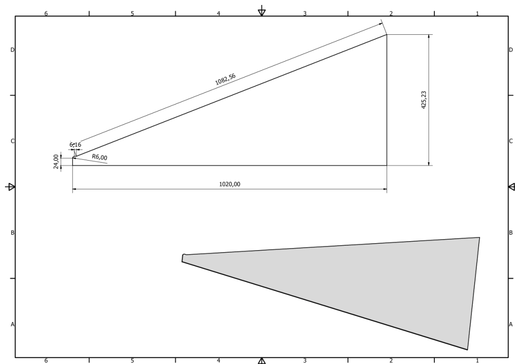
Figure 9 Triangle Sheet Working Drawing
