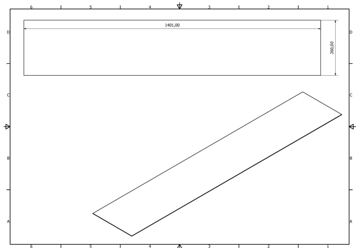
Figure 8 Top Base Sheet Working Drawing
