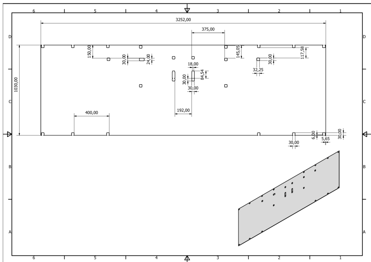
Figure 1 Base Sheet Working Drawing
