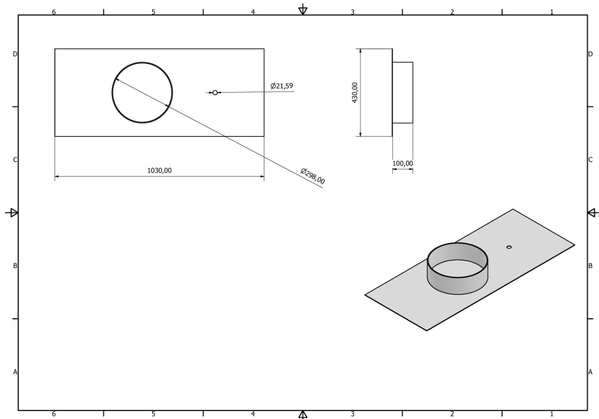
Figure 4 Mid Base 1 Sheet Working Drawing
