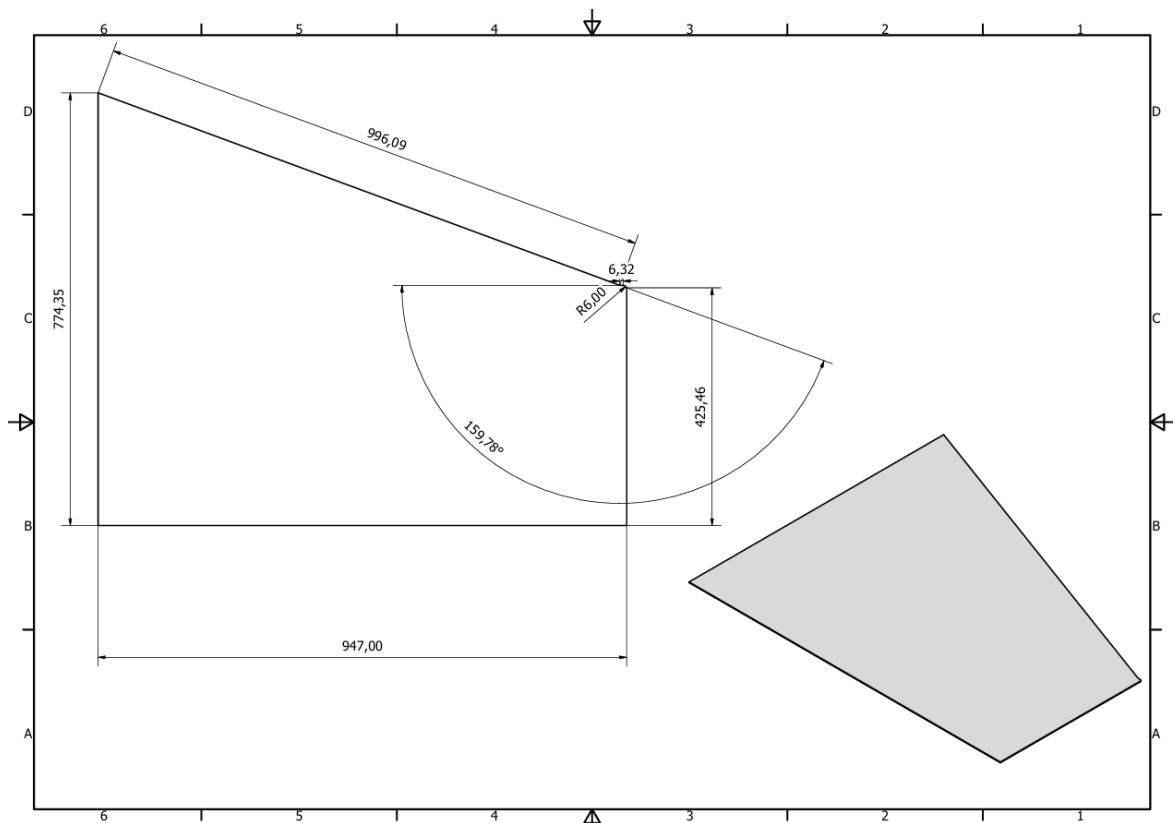
Figure 2 Side Sheet Working Drawing
